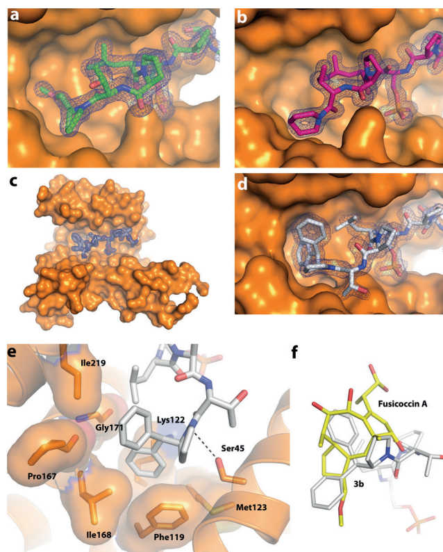
Figure 3. Binding of the chimeric inhibitors to 14-3-3 \sigma . Electron densities ( 2F_o - F_c , contoured at 1\sigma ) of 1b (a; green, blue, and red sticks, PDB No. 4Y32) and 2a (b; mauve and blue, PDB ID No. 4Y51) bound to 14-3-3 \sigma (orange solid surface). c) Electron density ( 2F_o - F_c , contoured at 1\sigma ) of 3b (white, blue, and red sticks, PDB No. 4Y3B) bound to 14-3-3 \sigma (orange solid surface). d) Enlarged view of (c). e) Residues of 14-3-3 \sigma directly accommodating modification of the Tau-pS214 recognition motif in 3b . Residues that contribute to the hydrophobic contact surface are shown as orange sticks with a semi-transparent surface and polar contacts as black dotted lines. f) Structural superposition of 3b (white sticks) and FC (yellow and red sticks) bound to 14-3-3 \sigma using PDB No. 3IQV as the template.
